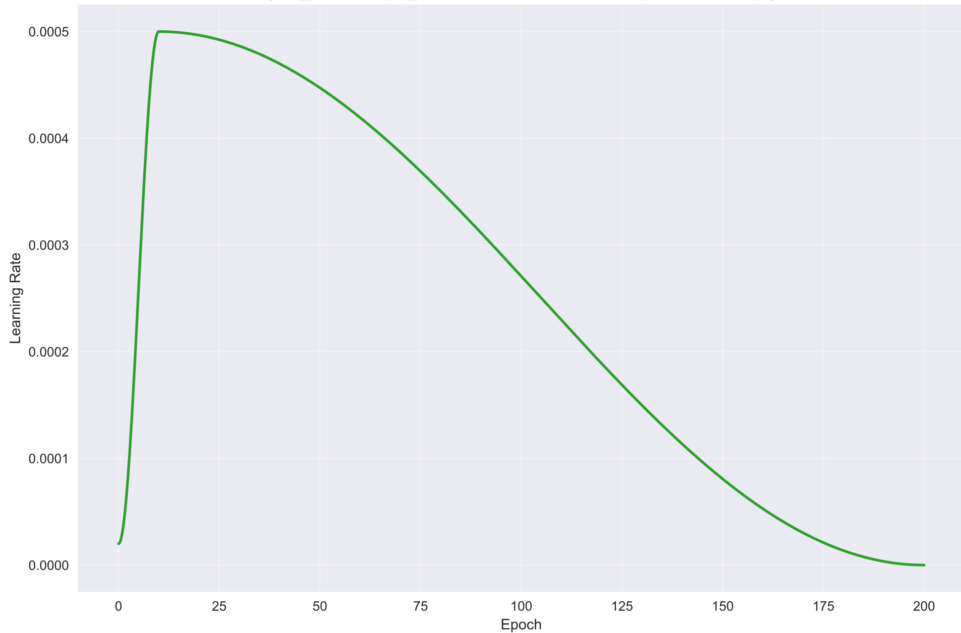
OneCycleLR Schedule — as configured in SSM/SSM.py (max_lr=0.0005, pct_start=0.05, cosine anneal, 200 epochs x 391 steps)
